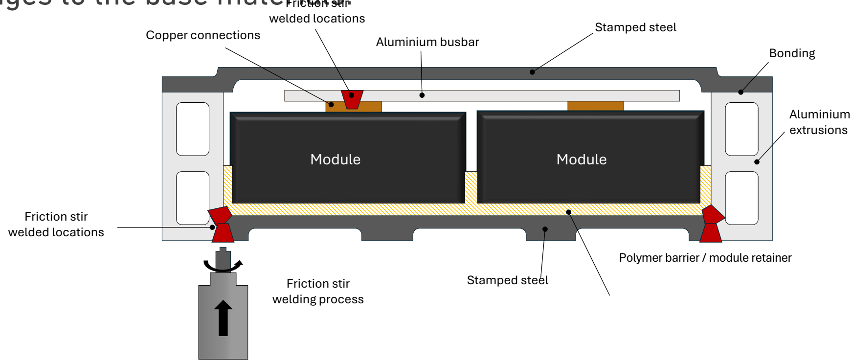
Figure 1 – Examples of multi material joints in modern vehicle batteries
