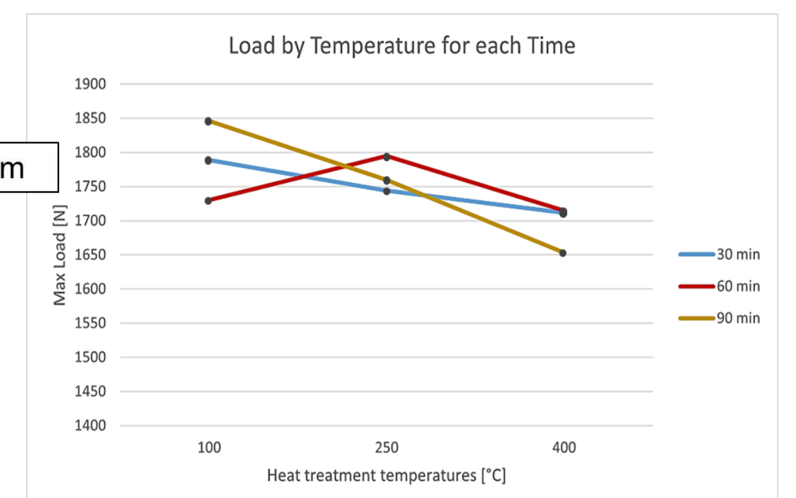
Figure 8 – Steel to aluminium specimens (left) and joint response to heat treatment temperatures and stage times (right)
